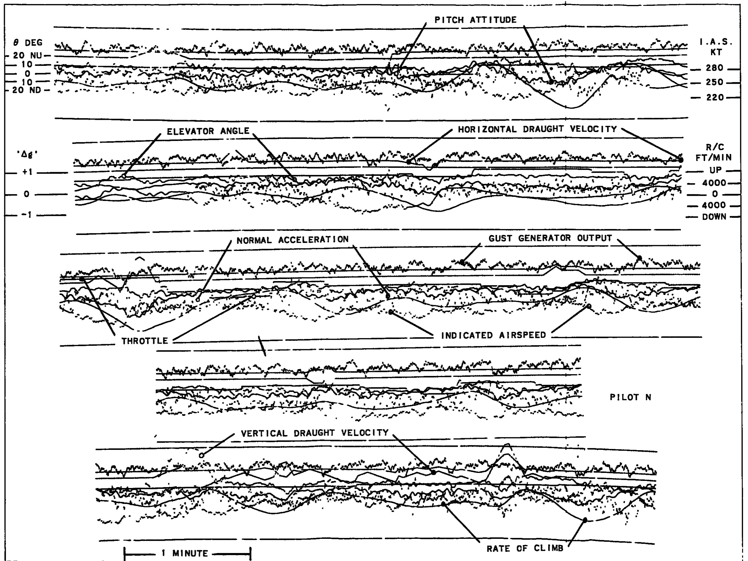
Fig.4e. Time history of a complete trial. Pilot N
