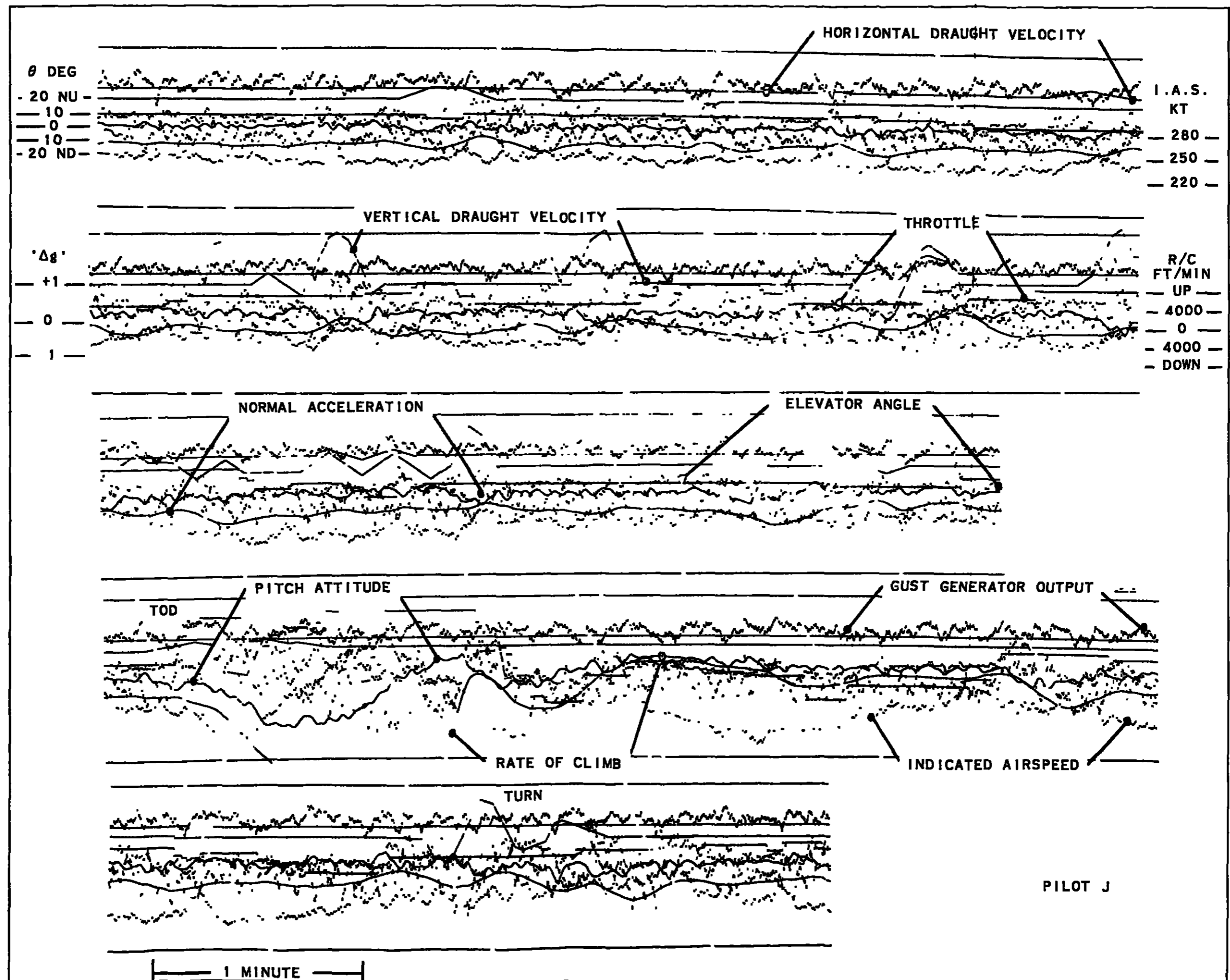
Fig.4c. Time history of a complete trial. Pilot J
