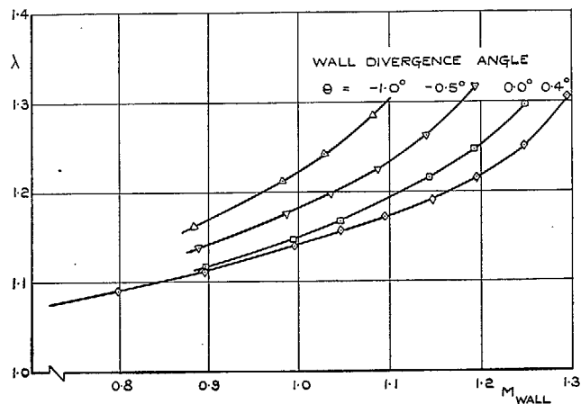
FIG. 16. Pressure ratio \lambda at various wall settings.
