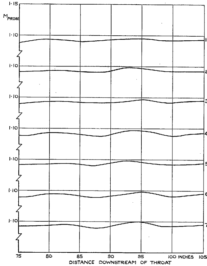
FIG. 12. Comparison of Mach number distributions on and off the centre-line. M_R = 1.1 , \theta = 0.25 deg.
