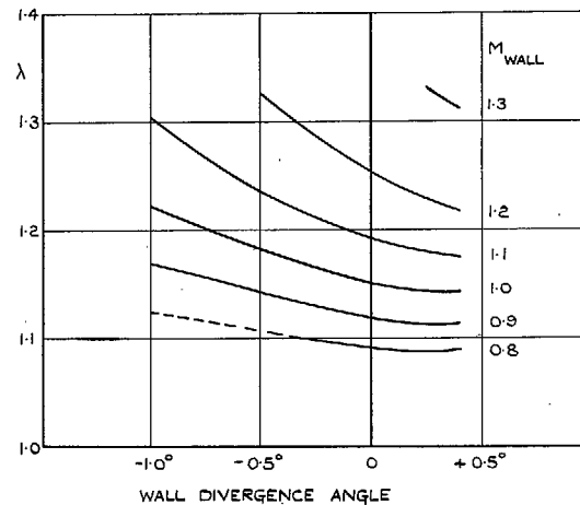
FIG. 17. Effect of wall inclination on pressure ratio.
