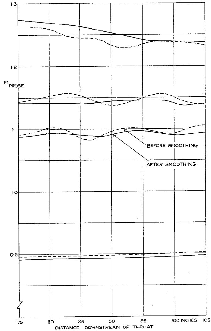
FIG. 10. Effect on centre-line Mach number distribution of smoothing working section walls. \theta = 0.25 deg.
