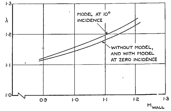
FIG. 19. Effect of a model on pressure ratio. \theta = 0.25 deg. (Model wing area 56 sq in., blockage 0.5 per cent.)
