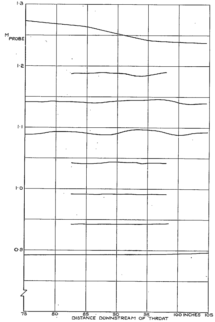
FIG. 9. Mach number distributions along tunnel centerline, from probe traverses. \theta = 0.25 deg.
