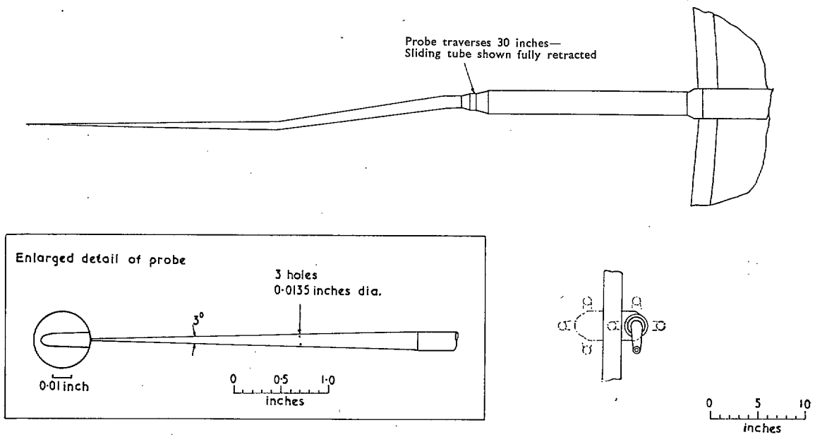
FIG. 4. Calibrating probe.
