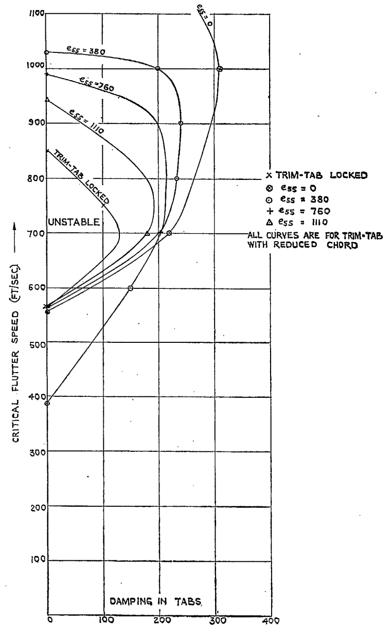
FIG. 12. Flutter speed vs. damping in tabs for various tab circuit stiffnesses.
