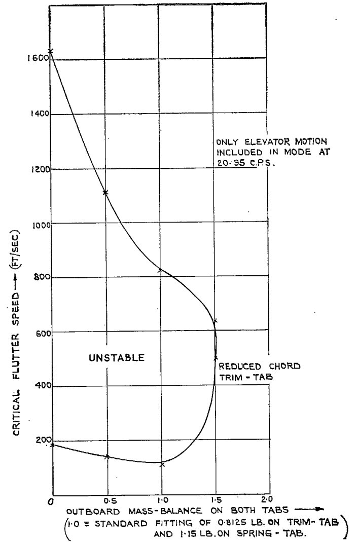
FIG. 10. Flutter speed vs. outboard mass-balance on both tabs. Antisymmetric case.
