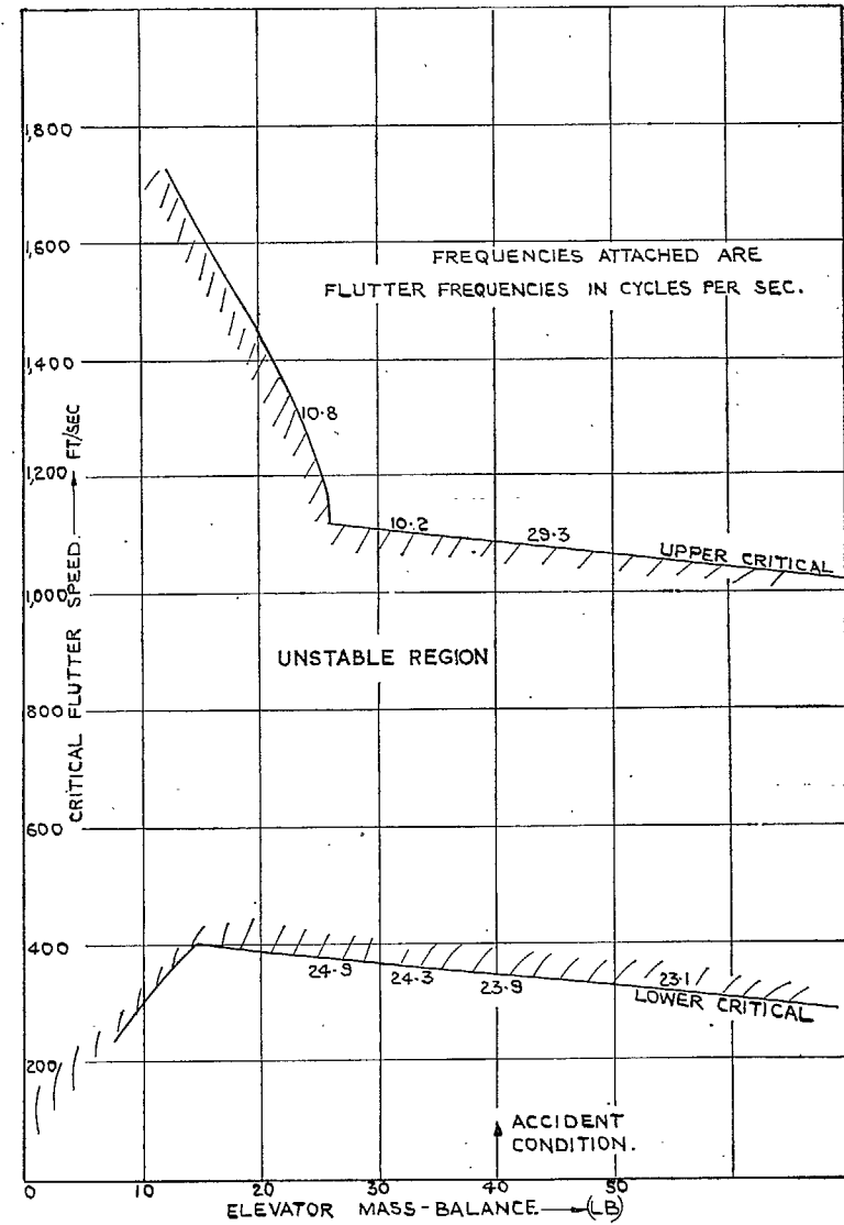
FIG. 6. Variation of flutter speed with elevator mass-balance.
