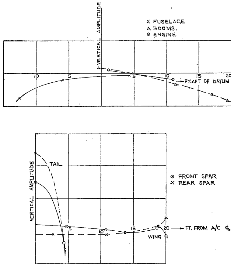
FIG. 5. Sea Venom symmetric ground resonance mode at 24.7 c.p.s. Vertical excitation at nose. Full internal fuel and forward tip-tank full.
