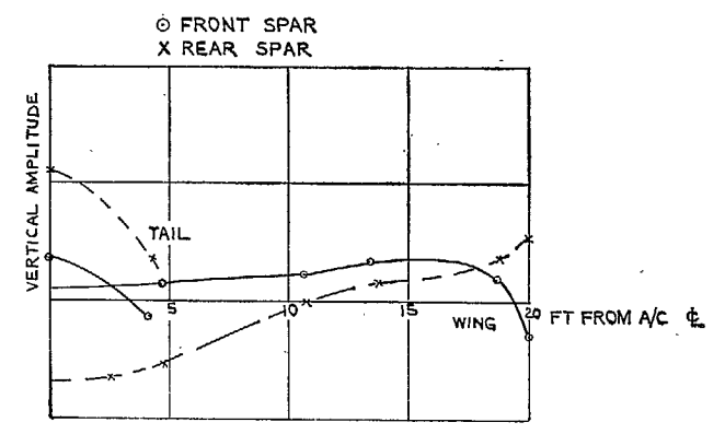
FIG. 4. Sea Venom symmetric ground resonance mode at 21.0 c.p.s. Vertical excitation at nose. Full internal fuel and forward tip-tank full.
