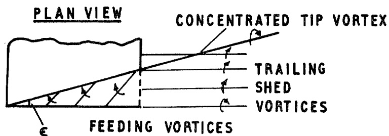
(C) CONCENTRATED TIP VORTEX METHOD
