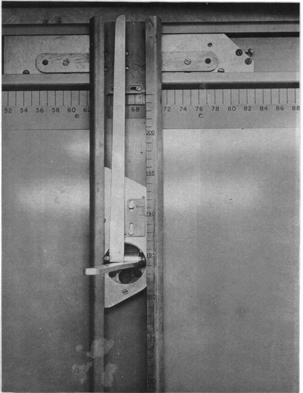
FIG. 7. Measuring probes in position for taking measurements from end wall.
