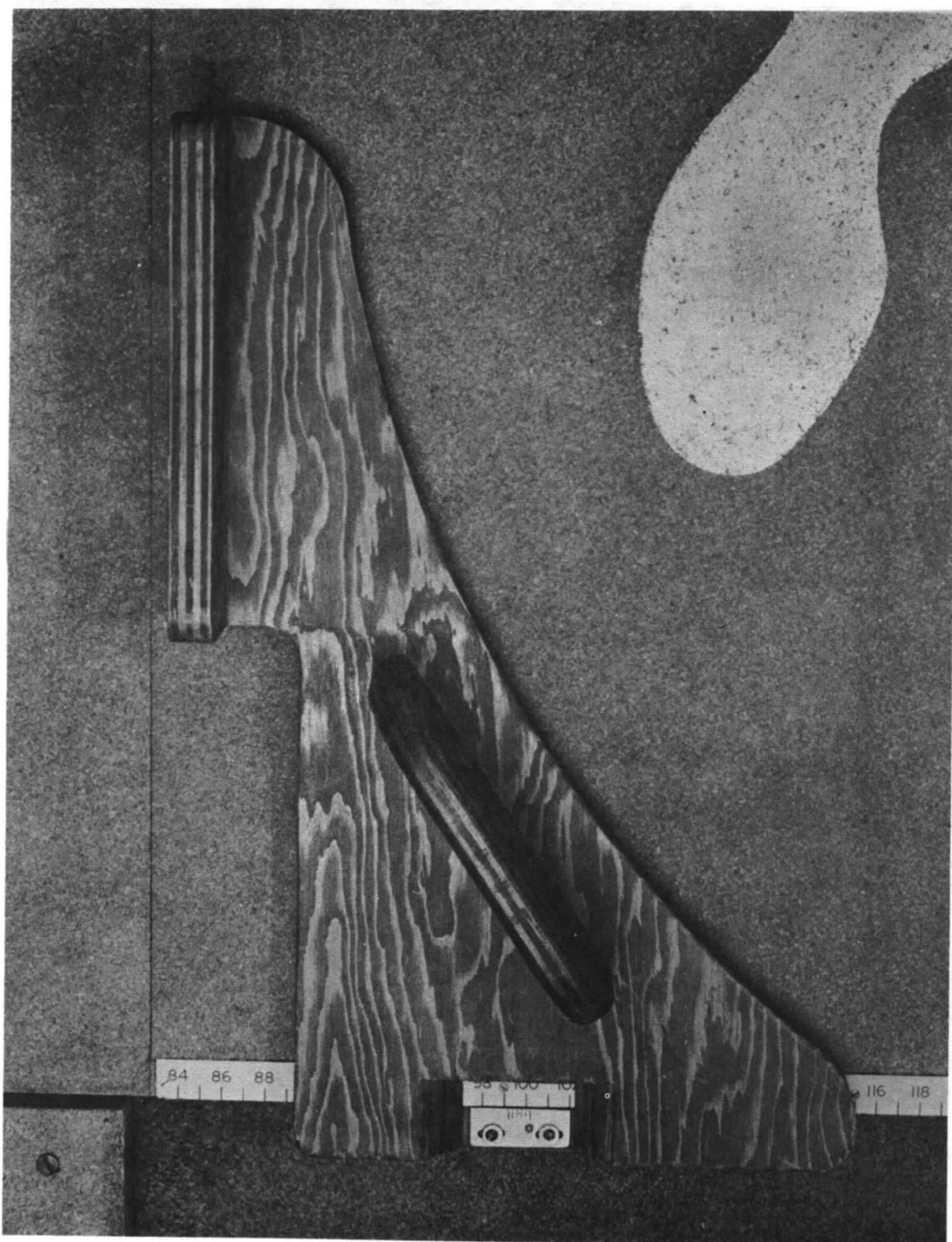
FIG. 9. Sliding block, for measuring buttock-heel length, positioned on scale inset on floor of measuring rig.
