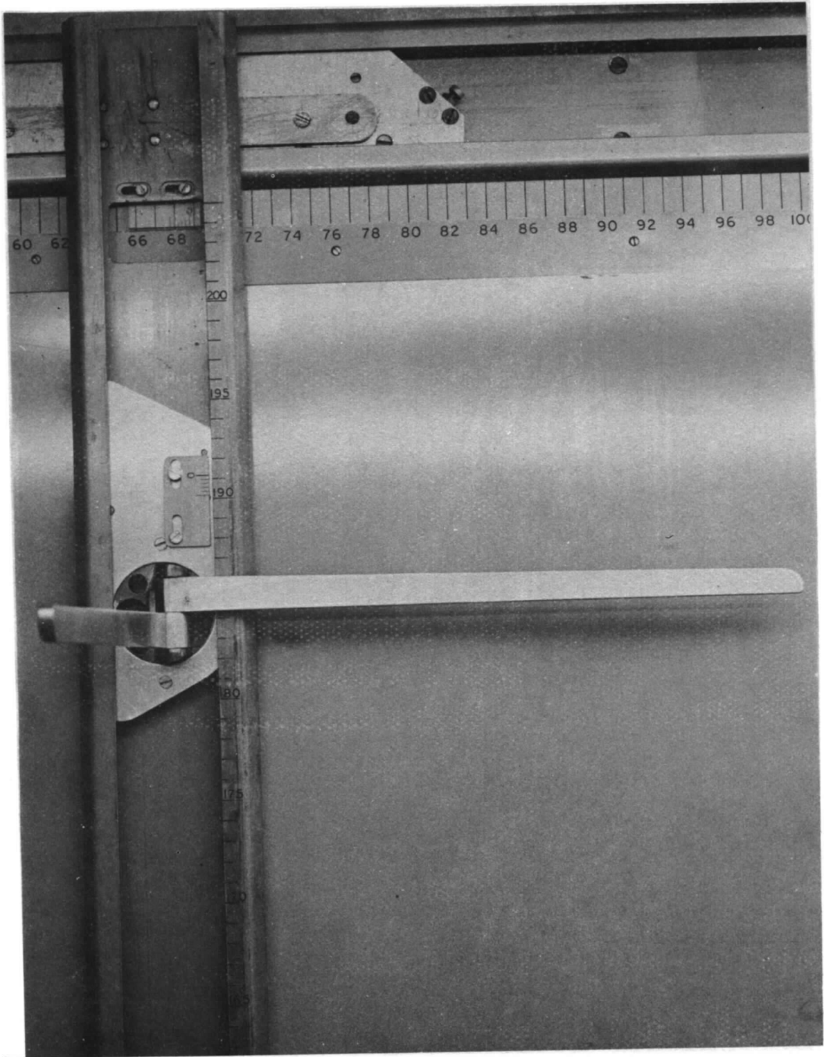
FIG. 8. Measuring probes in position for taking measurements from floor.
