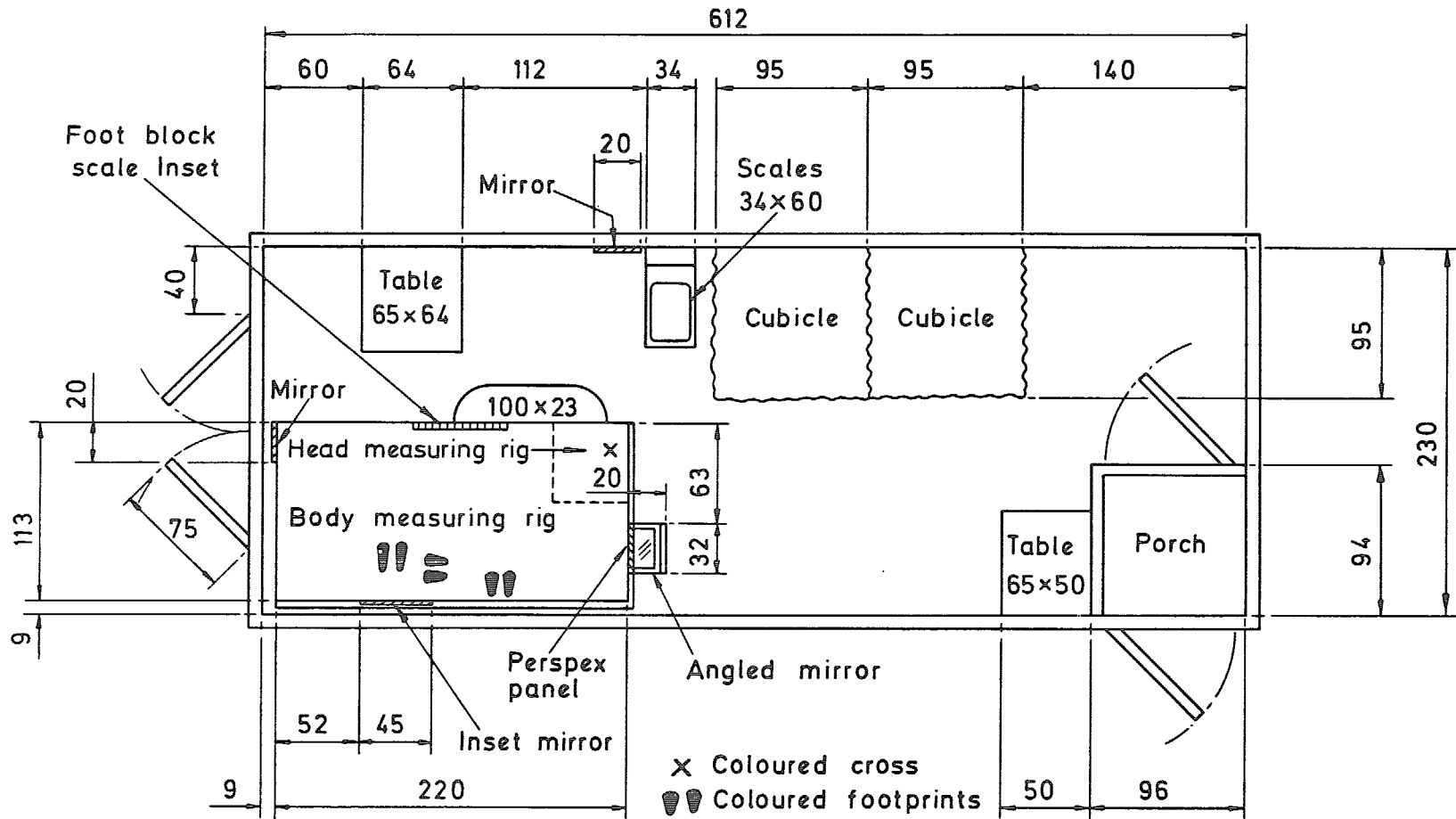
FIG. 3. Plan of mobile laboratory. Dimm. cm.
