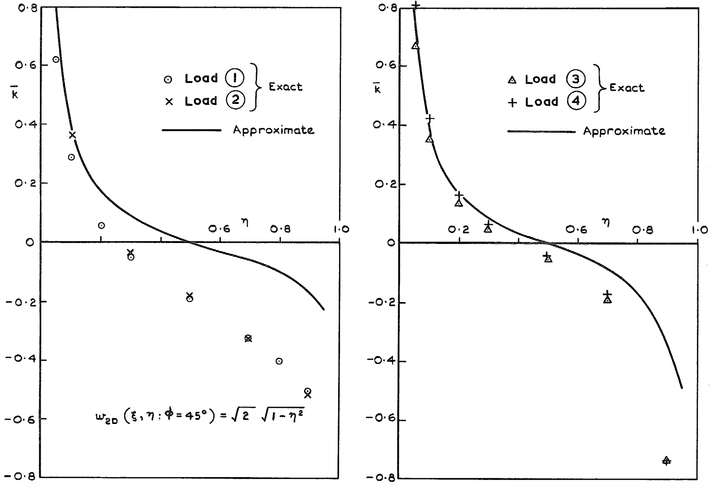
FIG. 20. The effect of sweep on the spanwise twist distribution \bar{k}(\eta) = \int_0^1 k(\xi, \eta) d\xi = \int_0^1 \{ [w - w_{2D}]_{\phi=45^\circ} - [w - w_{2D}]_{\phi=0^\circ} \} d\xi .
