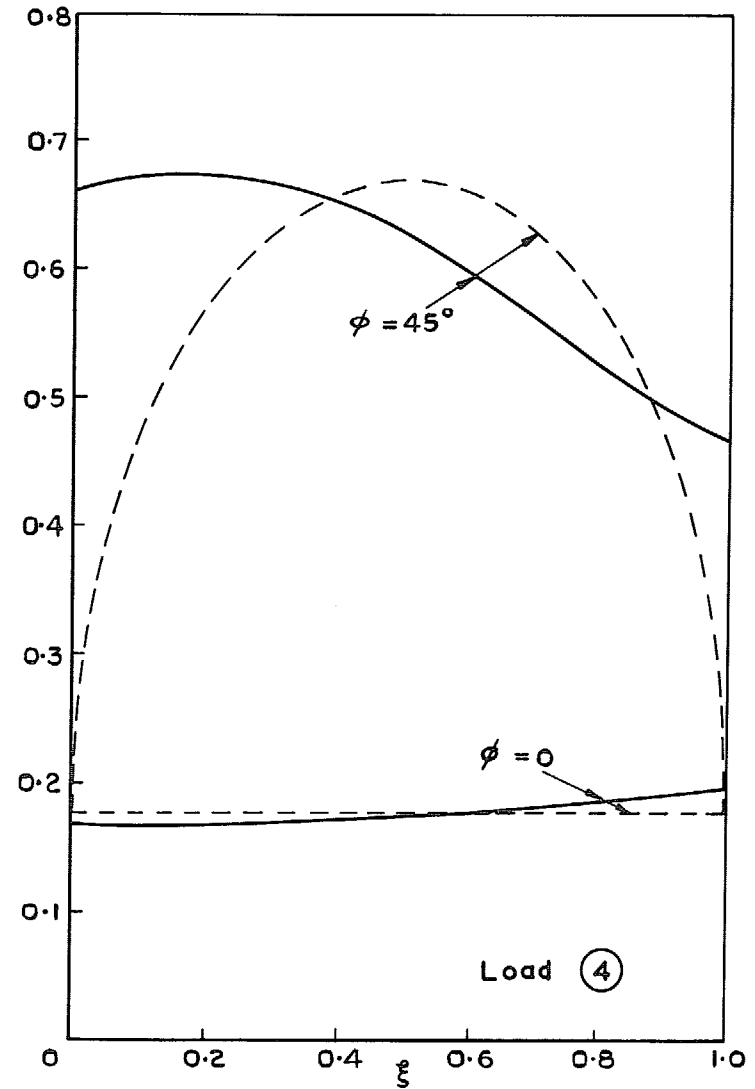
FIG. 12b. Threedimensional effect on downwash distributions at the inboard station \eta = 0.1 ; A = 6 .
