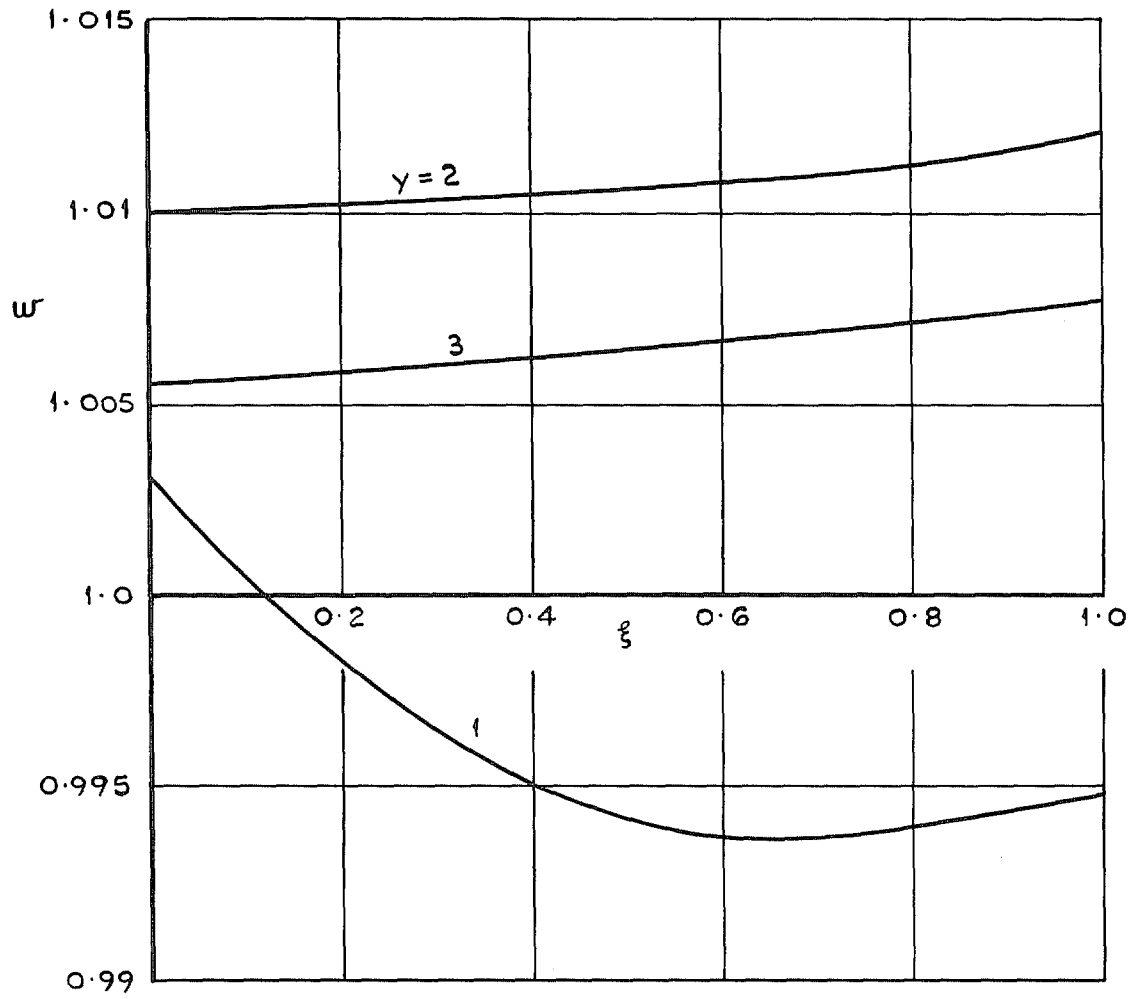
FIG. 26. Downwash related to the load distribution of equation (56) with C_l(y) from curve II of Fig. 25.
