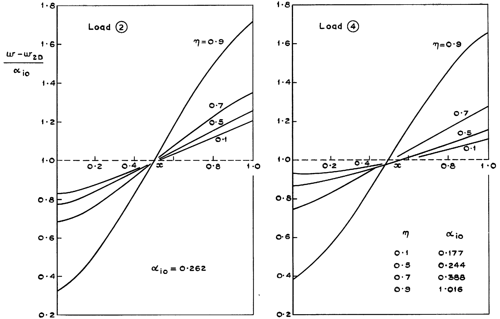
FIG. 9b. Threedimensional effect on downwash distributions for rectangular wings; A = 6 .
