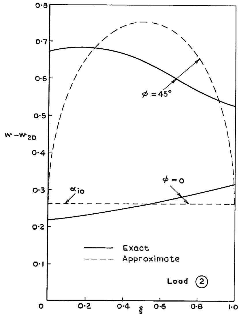
FIG. 12b. Threedimensional effect on downwash distributions at the inboard station \eta = 0.1 ; A = 6 .
