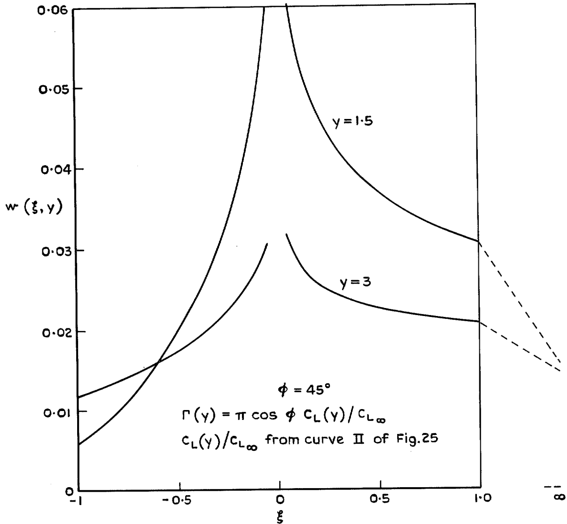
FIG. 27. Downwash induced by a trailing vortex sheet originating from a single swept spanwise vortex at x = |y| , -\infty < y < \infty of strength \Gamma(y) .
