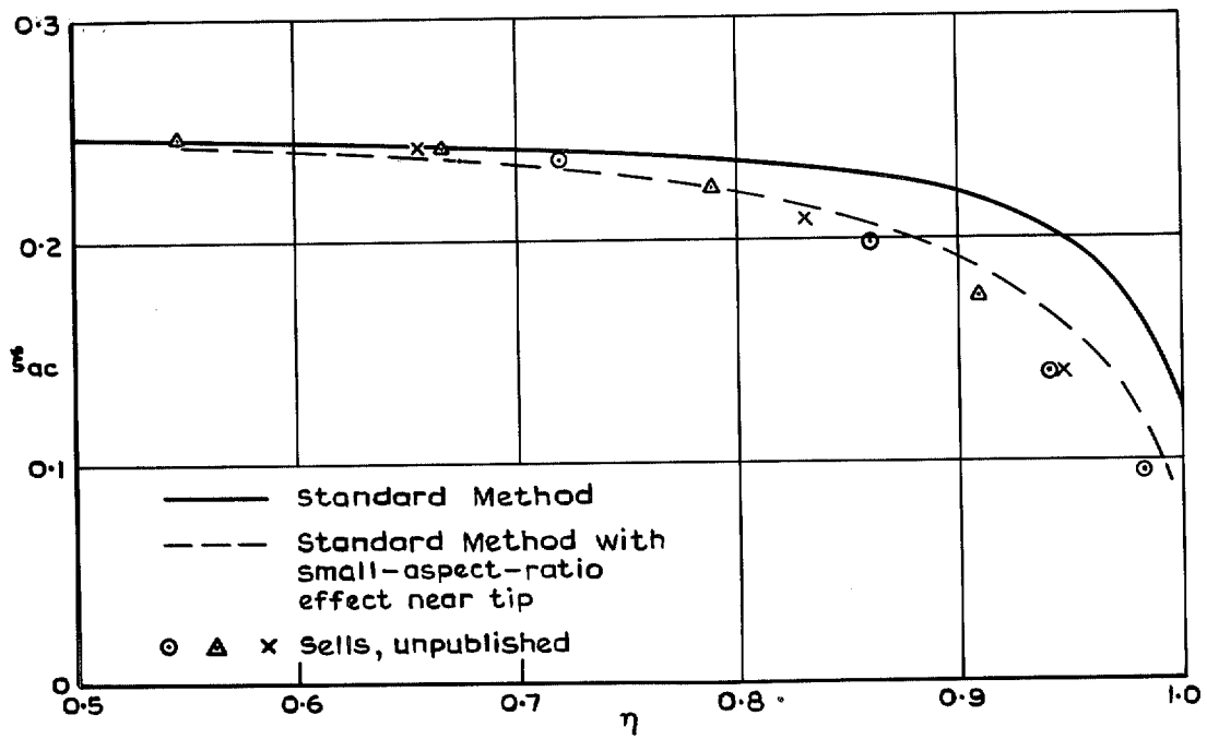
FIG. 31. Spanwise distribution of the position of the aerodynamic centre on a swept wing.
