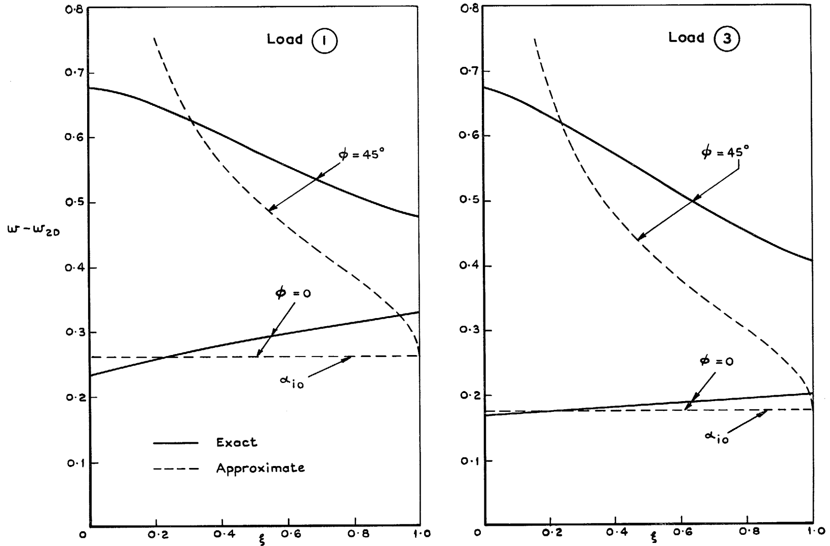
FIG. 12a. Threedimensional effect on downwash distributions at the inboard station \eta = 0.1 ; A = 6 .
