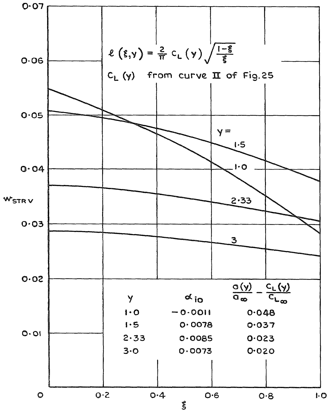
FIG. 28. Downwash induced by streamwise vorticity on infinite swept wing.
