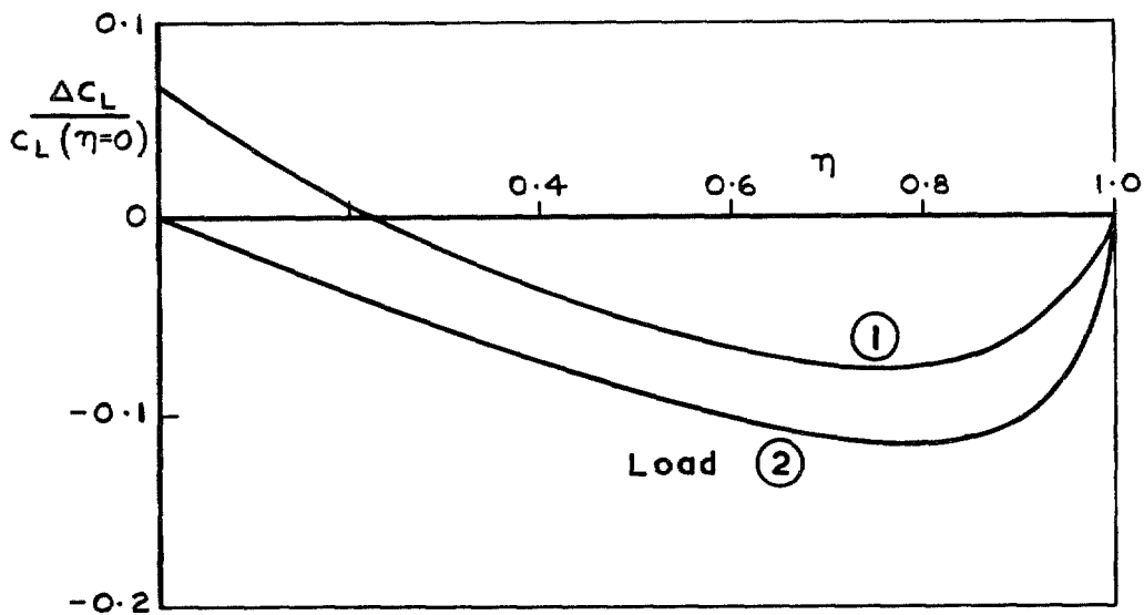
FIG. 33. C_L distribution for a swept wing with the slope \partial z(x, y)/\partial x = -w_{\text{exact}}(x, y) + w_{\text{approx}}(x, y) .
