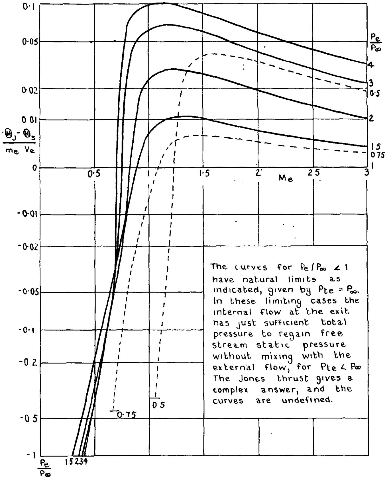
Curves of the difference between the Jones thrust and the standard thrust.
