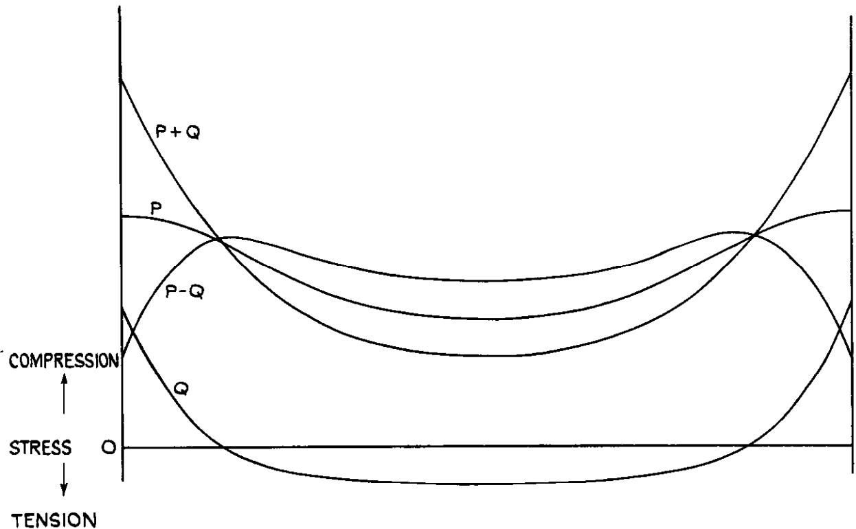
FIG. 35 SECTION OF STRESSES ON \phi .
