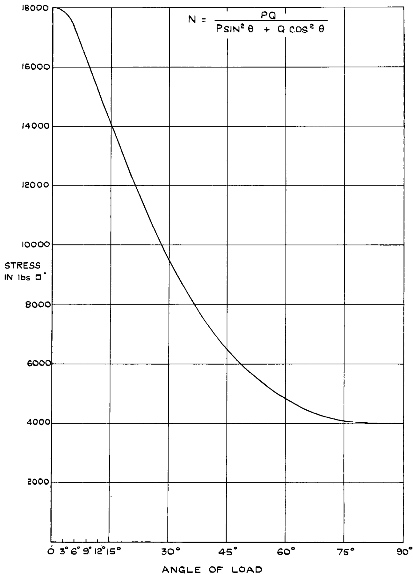
FIG.38 DURESTOS TENSION PROPERTIES THROUGH THE THICKNESS FOR ALL ANGLES OF LOADING.
