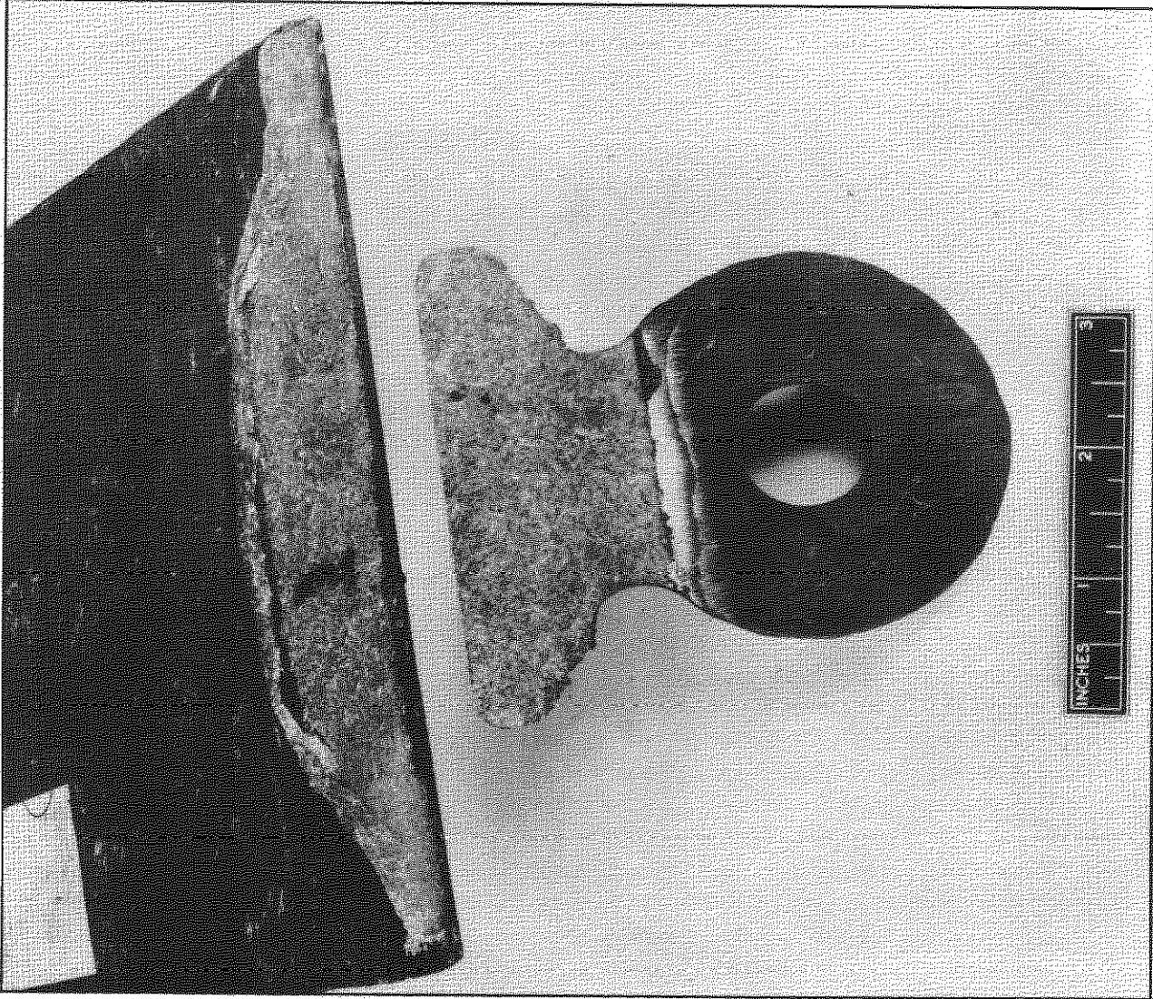
FIG.3c. SHEAR AND TENSION FAILURE AT 9.12 TONS
