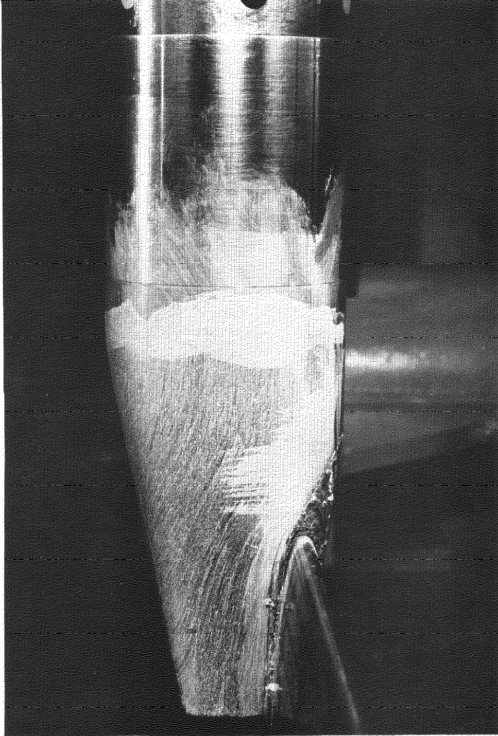
Fig.23. Oil flow on the nozzle at M_0 = 0.74 and H_j/p_0 = 2.4
