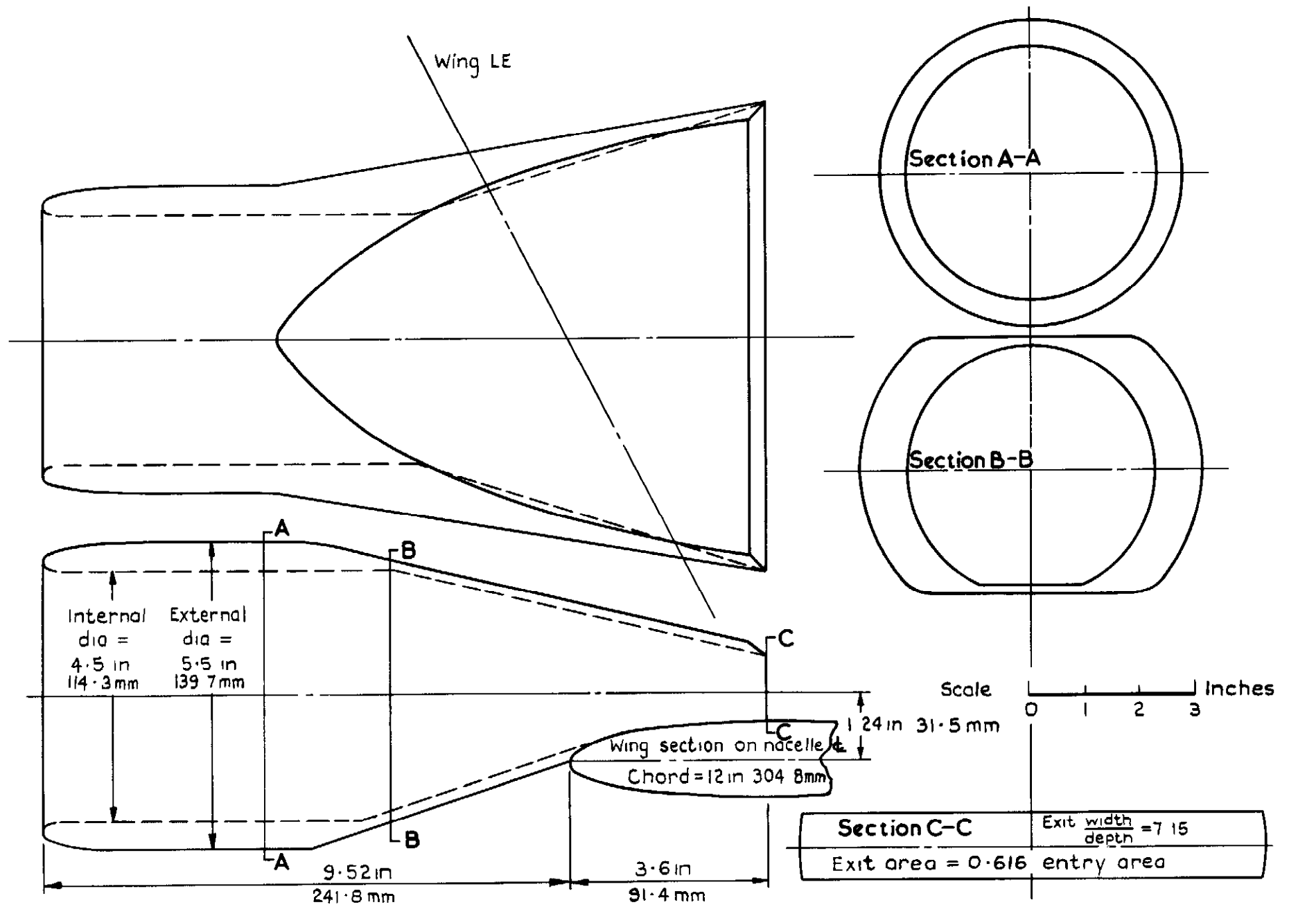
Fig. 27 Overwing nacelle 'B' - flored width
