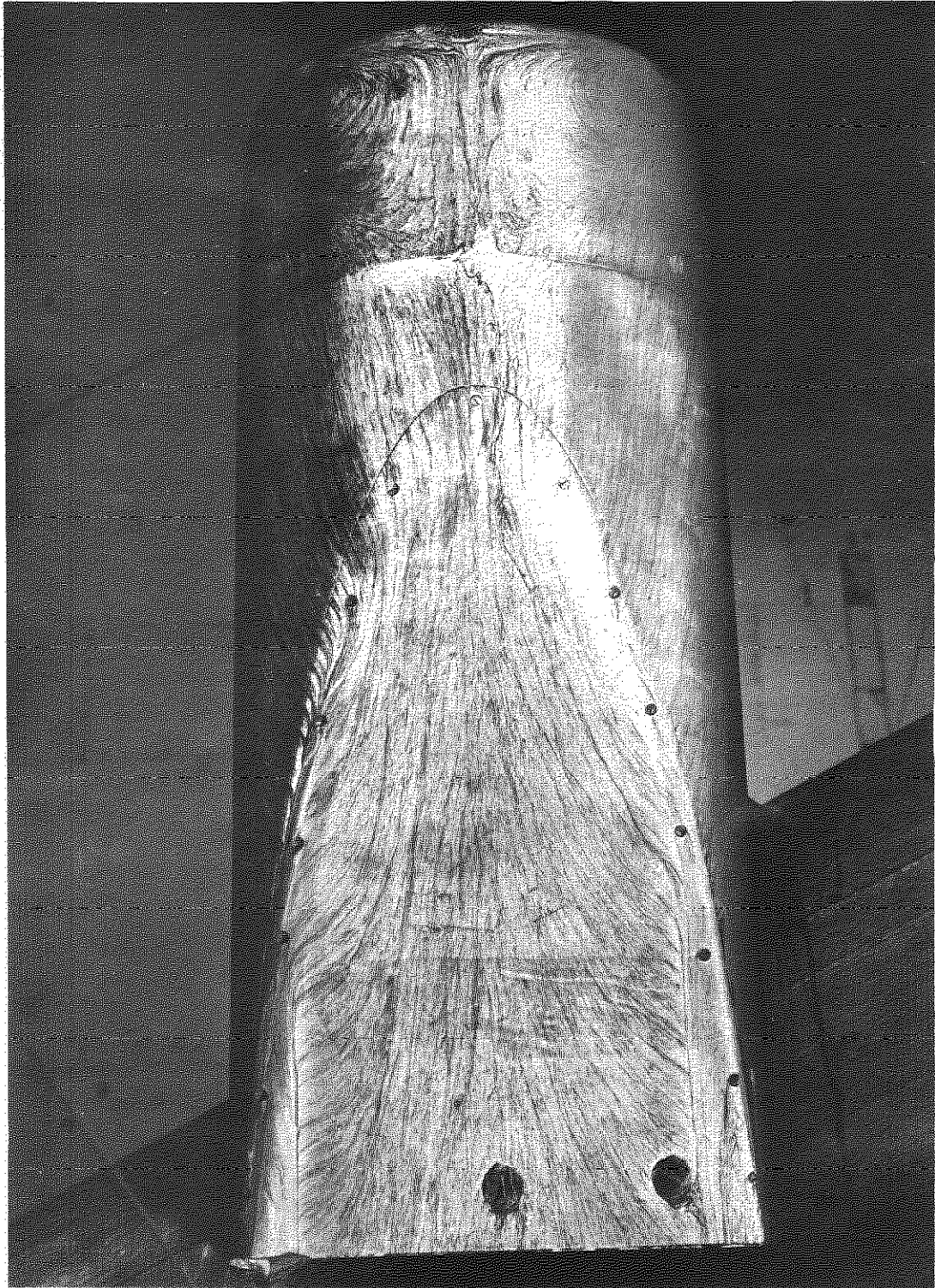
Fig.36. Flow visualization on upper surface of nacelle A; \alpha_w = 9^\circ
