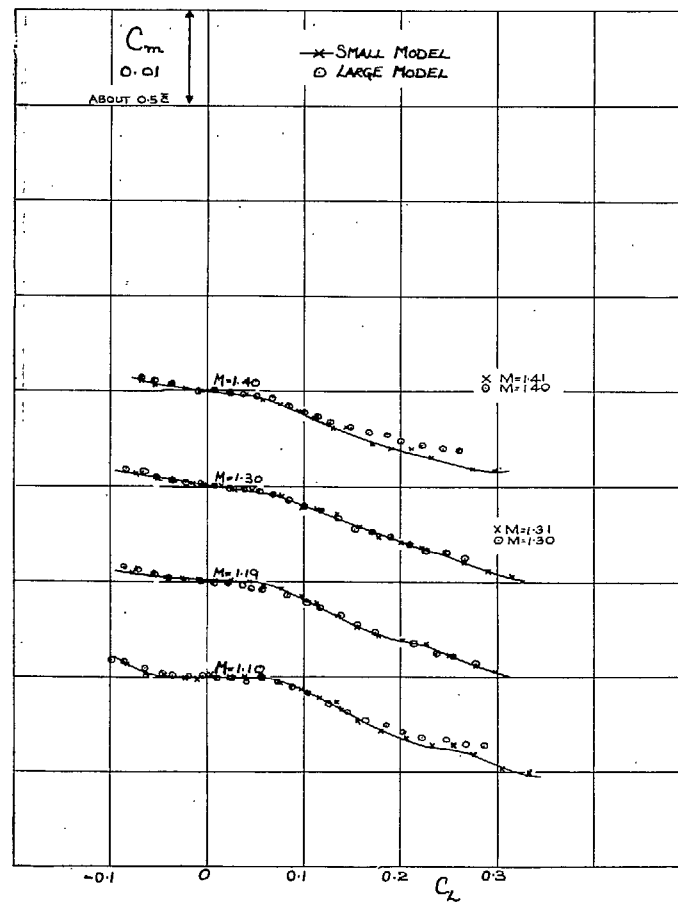
FIG. 3b. Pitching-moment curves. M = 1.1 to M = 1.4 .
