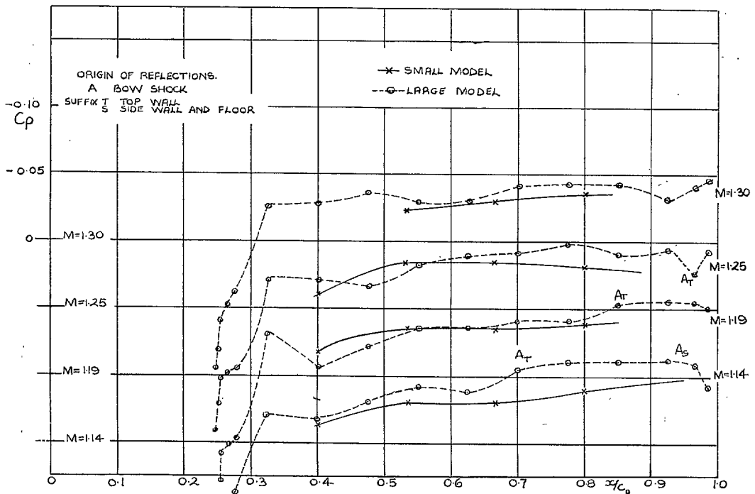
FIG. 12b. Chordwise C_p distributions. \eta = 0.25 .
