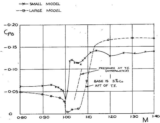
FIG. 7. Variation of base pressure with Mach number.
