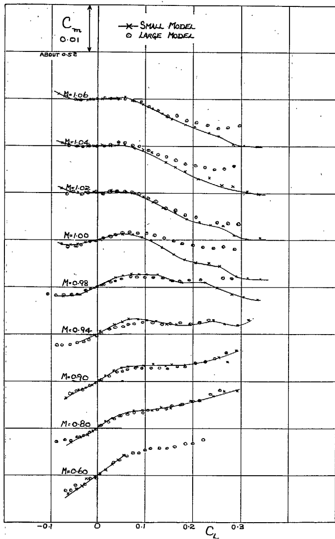
FIG. 3a. Pitching-moment curves. M = 0.60 to M = 1.06 .
