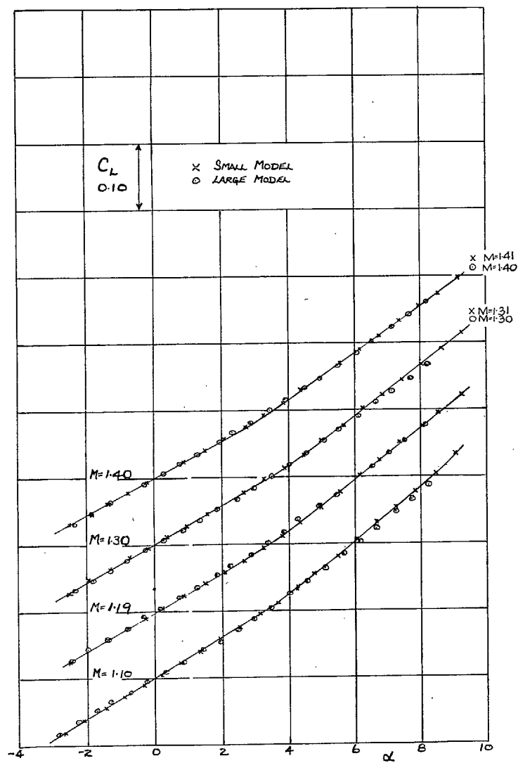
FIG. 2c. Lift curves. M = 1.1 to M = 1.4 .
