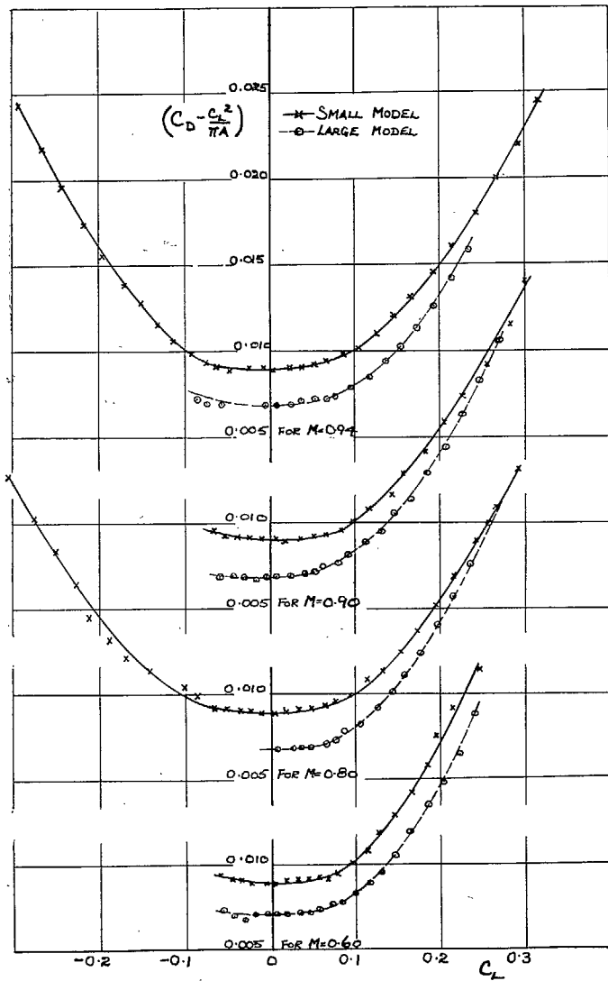
FIG. 4a. Variation of (C_D - C_L^2 / \pi A) with lift. M = 0.60 to M = 0.94 .
