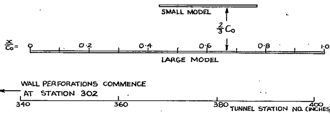
FIG. 1d. Longitudinal positions of models and properties of perforated walls.
