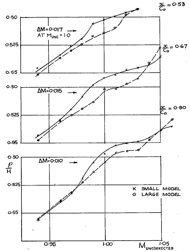
FIG. 9b. Variation of p/H with Mach number, \eta = 0.45 .
