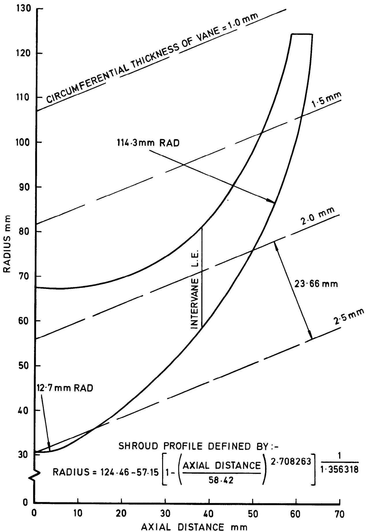
FIG. 3 IMPELLER MERIDIONAL SHAPE AND VANE THICKNESS
