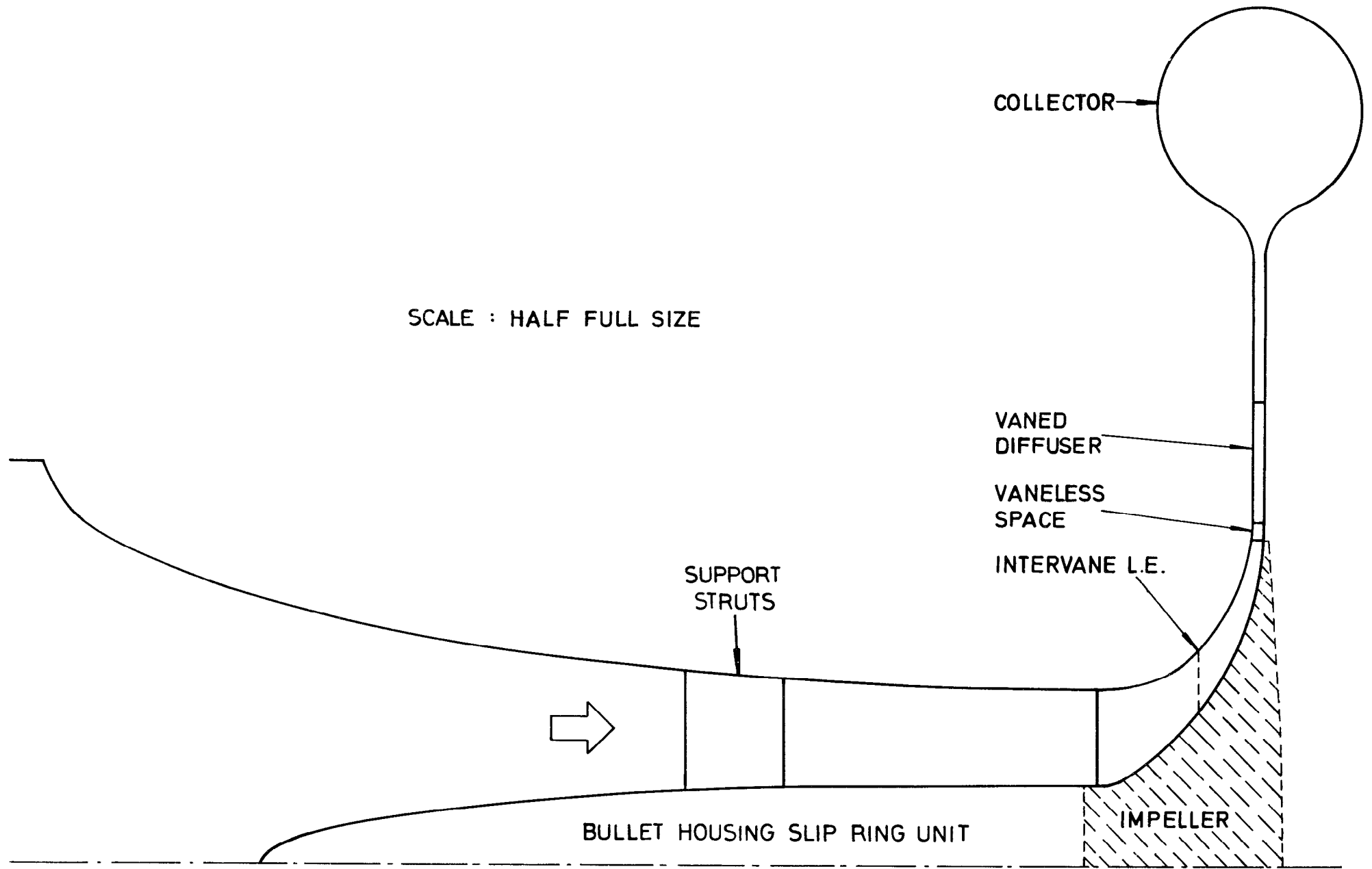
FIG.1 LAYOUT OF COMPRESSOR
