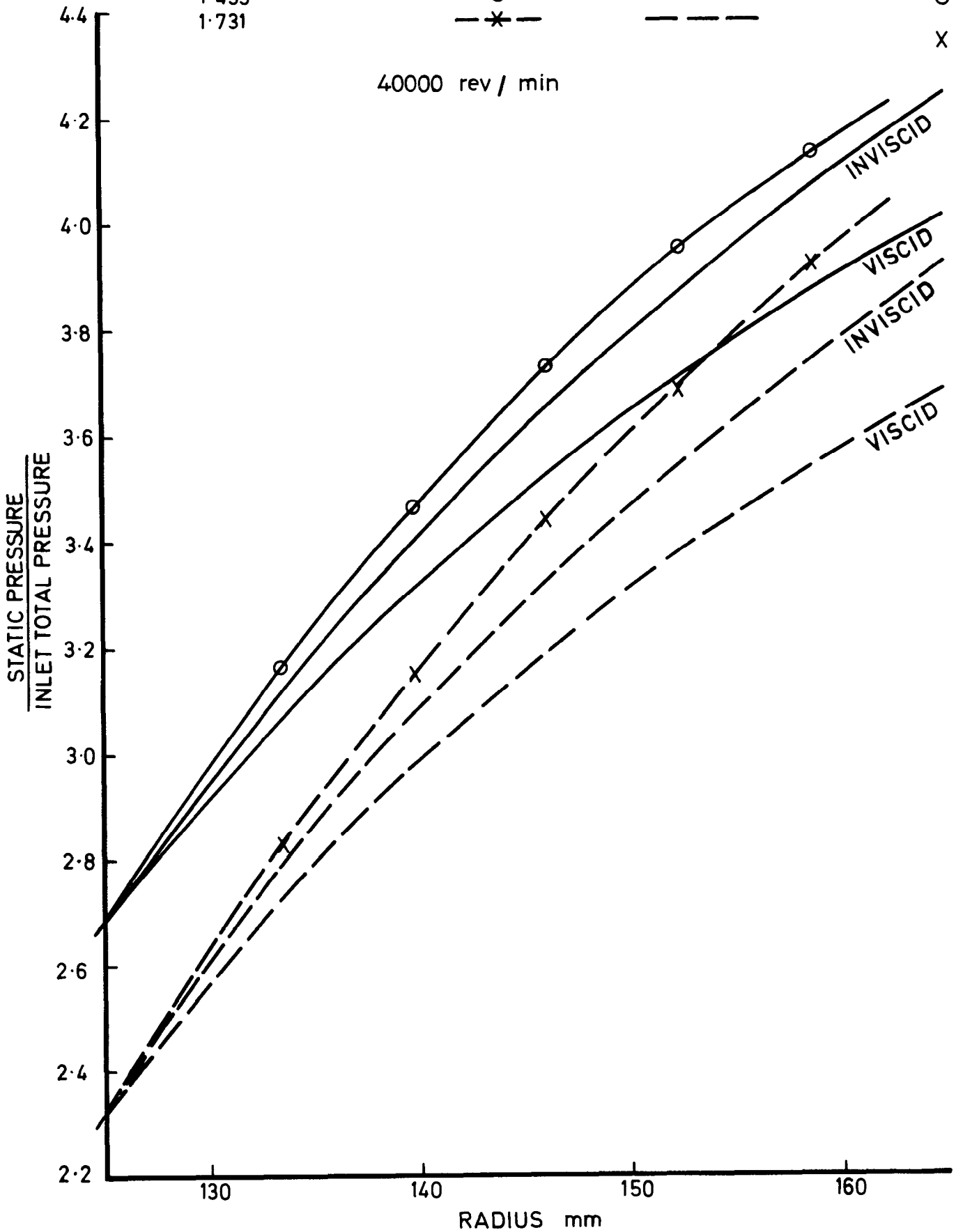
FIG.22 BUILD V VANELESS DIFFUSER AREA-WEIGHTED MEAN STATIC PRESSURES
