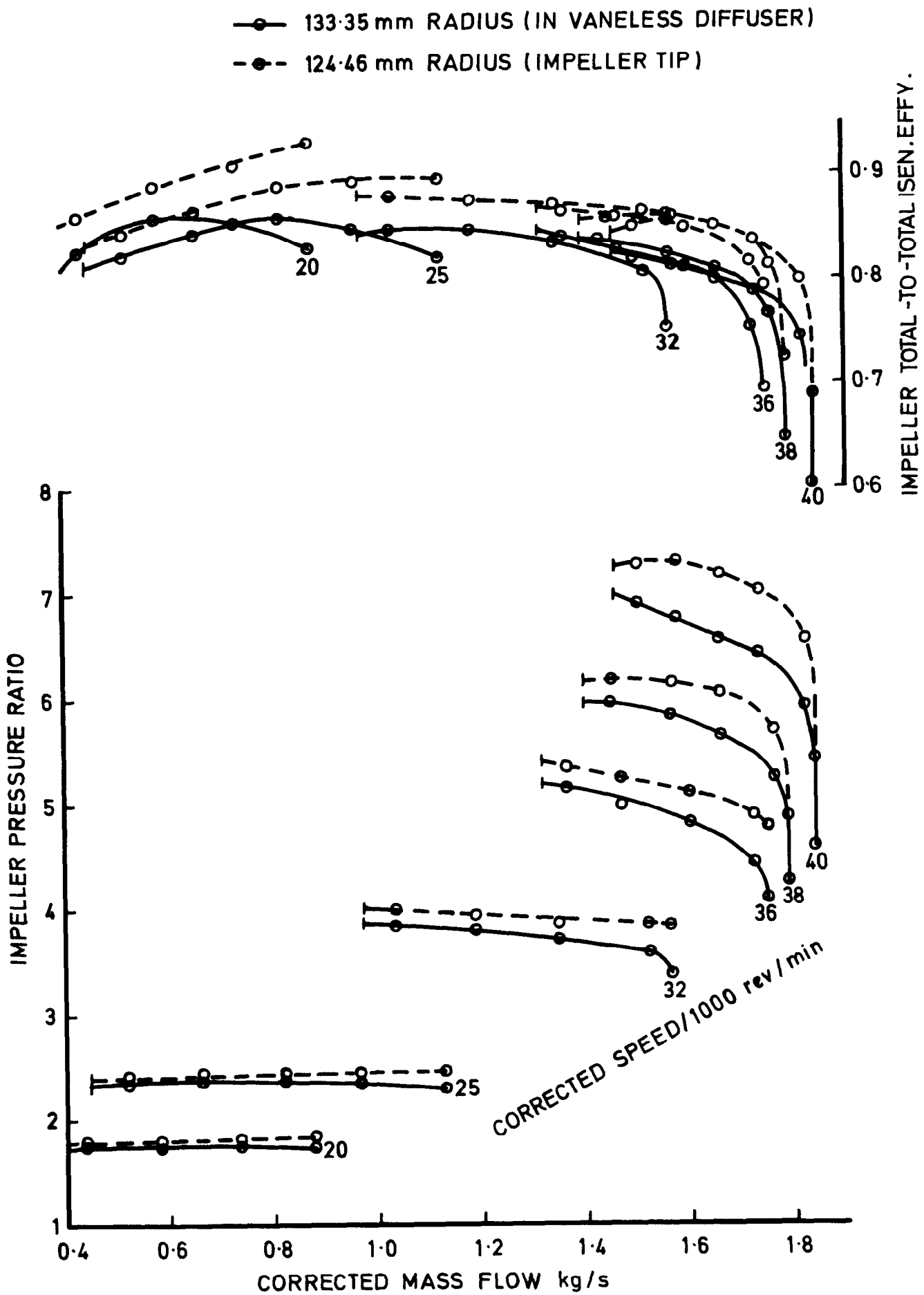
FIG.12 BUILD V IMPELLER CHARACTERISTIC
