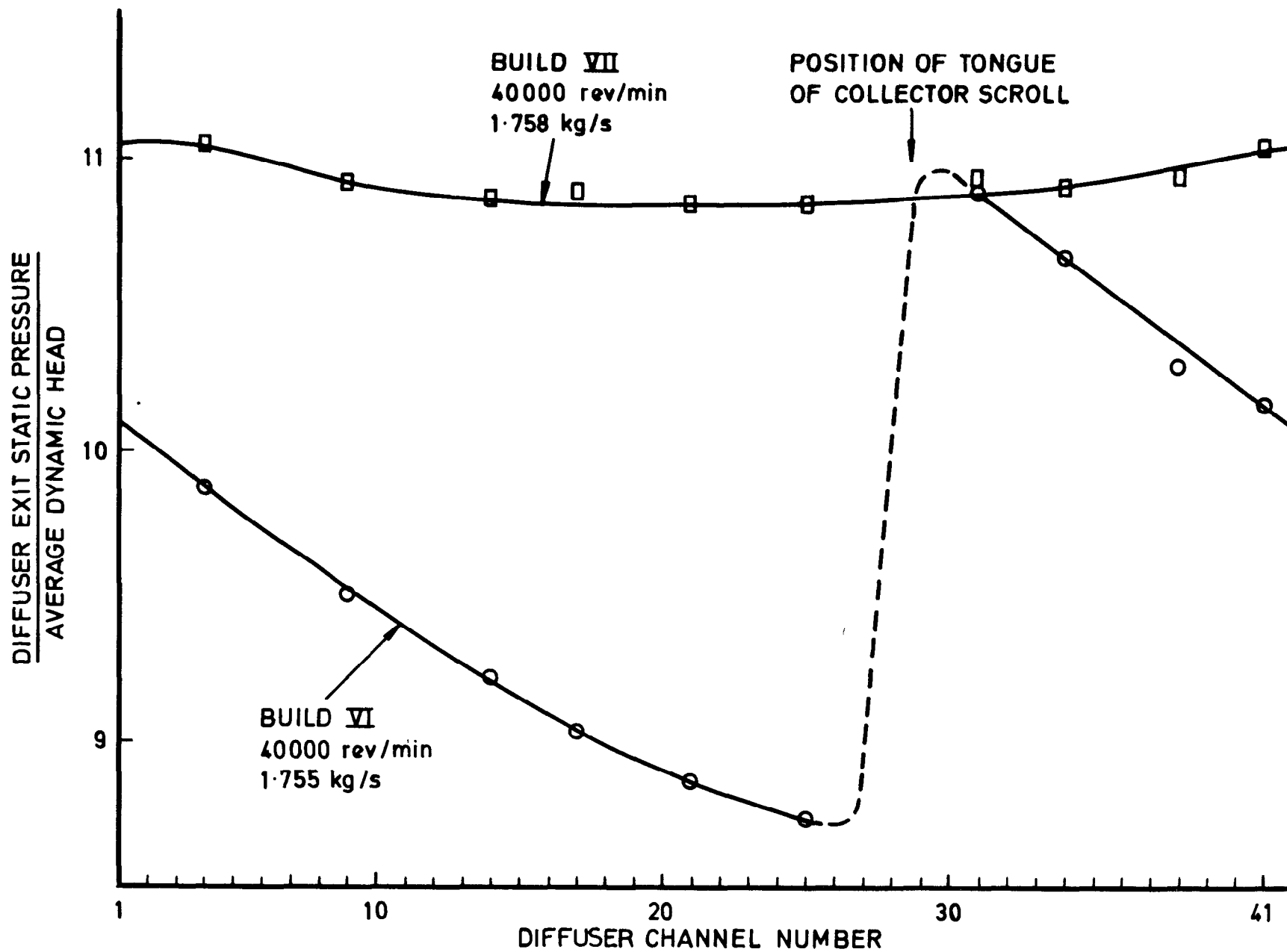
FIG. 14 VARIATION OF STATIC PRESSURE AT DIFFUSER EXIT
